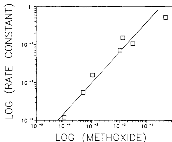
Figure 7. First-order rate constants for the reaction of \text{PdBr}(\text{COC}_6\text{H}_5)_2(\text{P}(\text{C}_6\text{H}_5)_3)_2 at 90 °C with 1 M methanol and a variety of 1 M amines as a function of the resulting estimated methoxide ion concentration (calculated on the basis of amine \text{p}K_a values in water).
